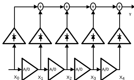
Figure 21. Logarithmic Amplifier
